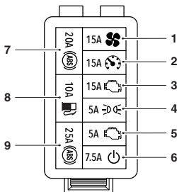
Trident Fuse Box 1
