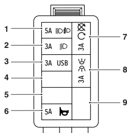
Tiger Sport Fuse Box 2
