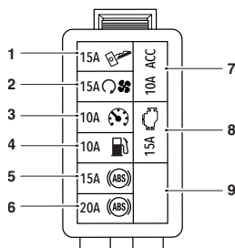
Tiger Sport Fuse Box 1
